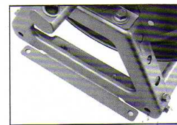
Optional External Mounting Brackets part no. 9906.0027. Add 2-1/2" to the X dimensions shown in the chart.
